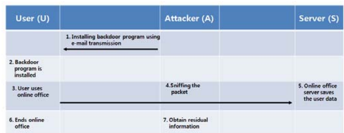
Fig. 1 Attack Scenario
