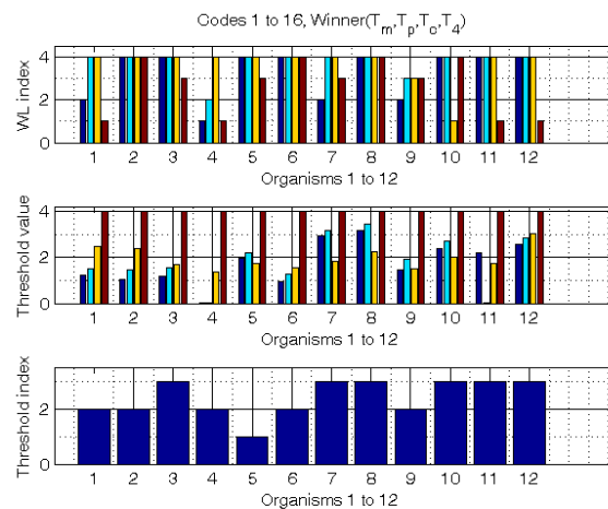
Fig. 2 WL index (top), threshold value (middle), and threshold index (bottom) of top classifications of 12 organisms
