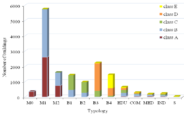
Fig. 8 Distribution of vulnerability classes into each typology
