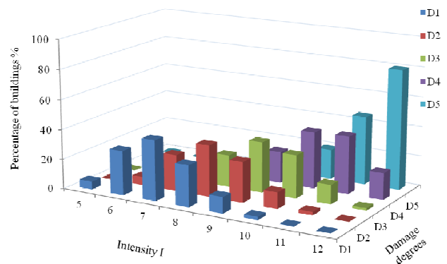
Fig. 10 Distributions of damage degrees for different intensities
