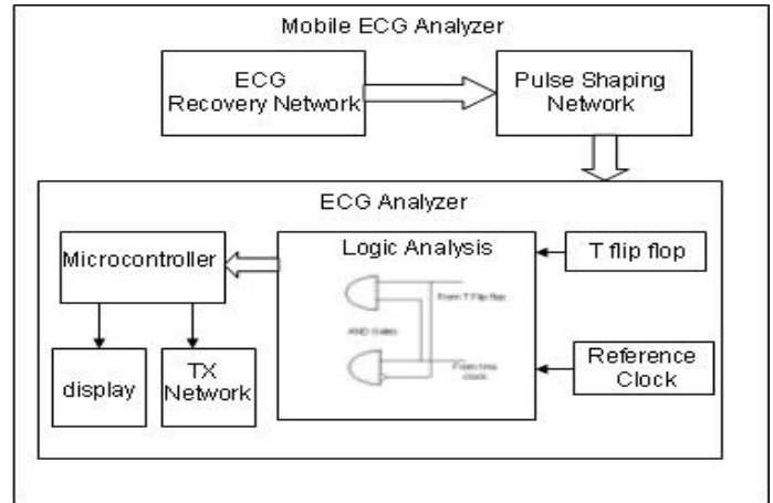
Fig. 4 Essential blocks of Mobile ECG Analyzer
