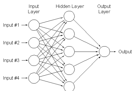
Fig. 5 Basic structure of a Feed Forward Network
