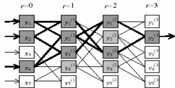
Fig. 3 Polynomial Neural Network trained by GMDH Algorithm
