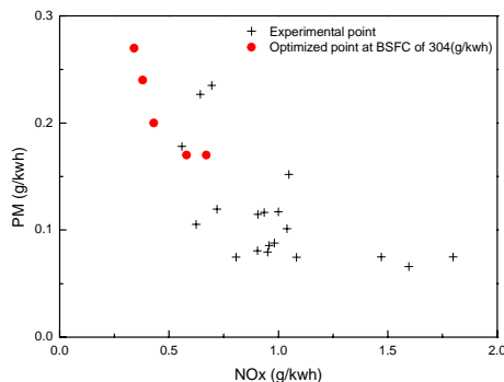
Fig. 11 Experimental and optimized points on BSNO x and BSPM map
