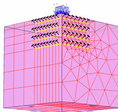
Fig. 2 3D modeling created with Plaxis3DT Bearing Stress (kPa)
