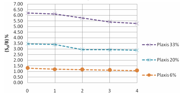
Fig. 7 Variation of (S_d/B) with number of reinforcement layers with geogrid
