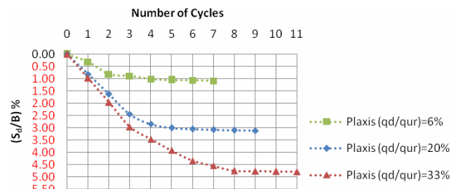
Fig. 6 .Variation of (S_d/B) with number of load cycles for series C10-C12
