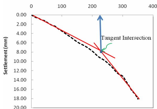
Fig. 3 Load settlement curve for unreinforced soil
