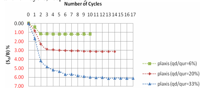
Fig. 5 .Variation of (S_d/B) with number of load cycles for Series B1-B3
