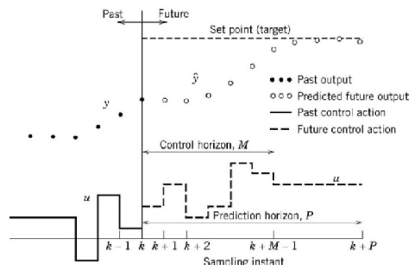
Fig. 1 Basic Concept for Model Predictive Control
