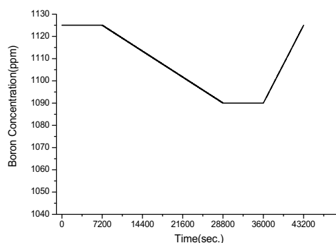
Fig. 3 Boron concentration change for a daily load-following operation
