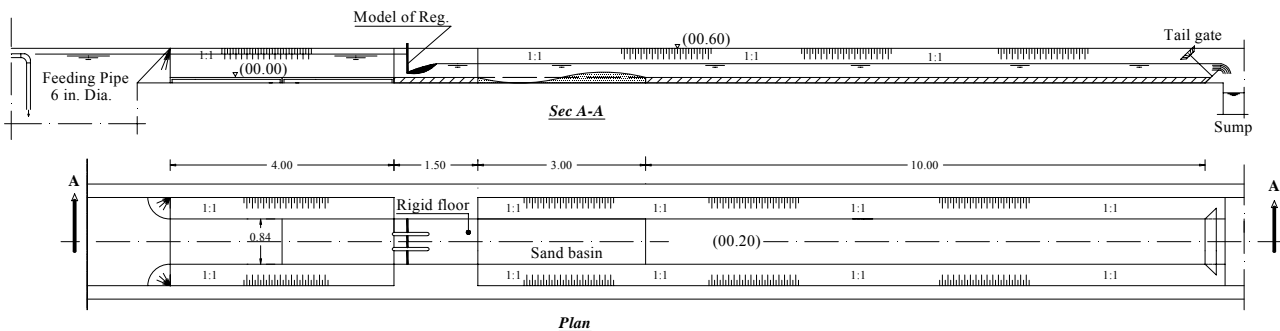
Fig. 2 Different parts of the experimental channel
