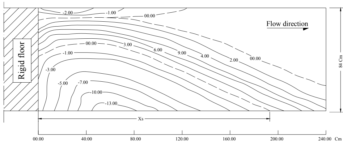
Fig. 9 Contour lines of the movable bed showing the scour hole profile behind rigid floor of length, L = 0.60 m for asymmetrical under-gated regulation ( H = 0.16 , Q = 21 Lit./s and h_g = 43 mm)
