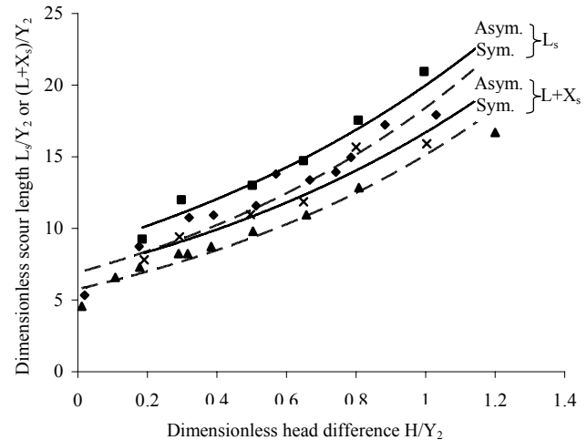
Fig. 5 Variation of L_s/Y_2 or (L+X_s)/Y_2 with H/Y_2 for symmetrical and asymmetrical under-gated regulations (submerged case)
