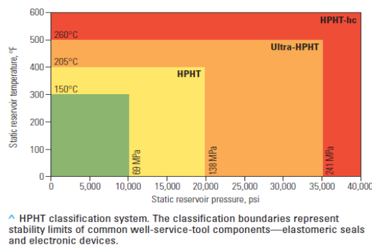
Fig. 1 HPHT classification
