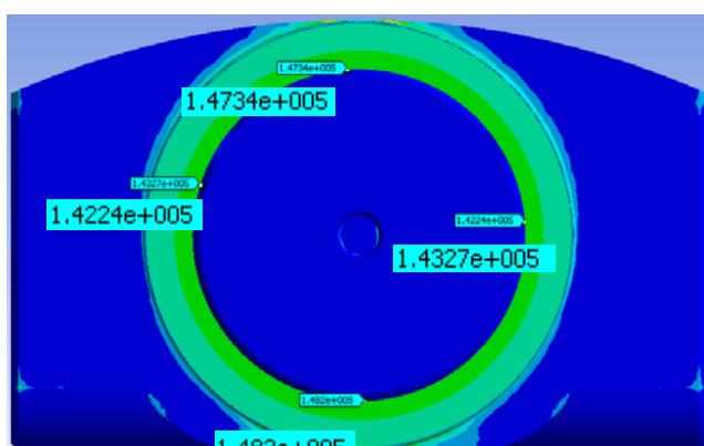
Fig. 7 von-Mises stress distribution
