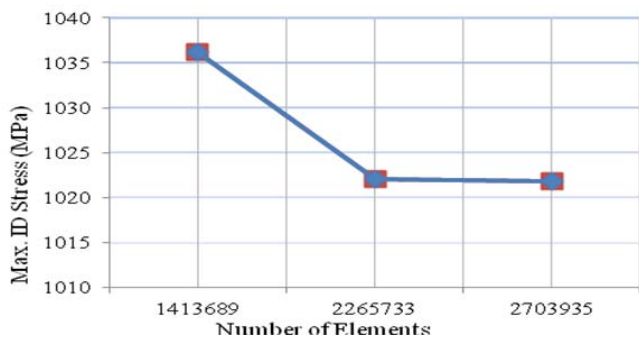
Fig. 4 Mesh sensitivity/independent check
