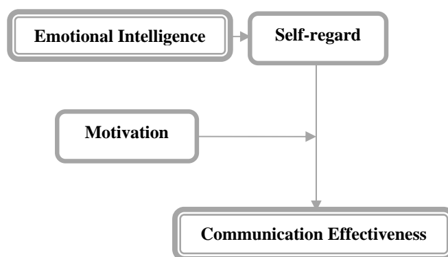
Fig. 2 Conceptual Framework
