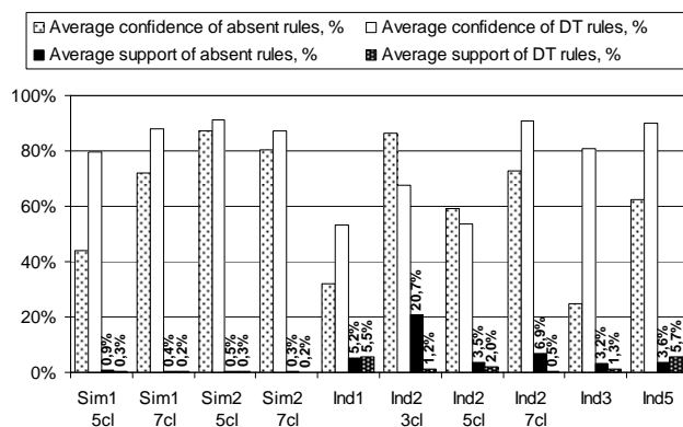
Fig. 6 Quality parameters of rules obtained from RST and omitted by DTs
