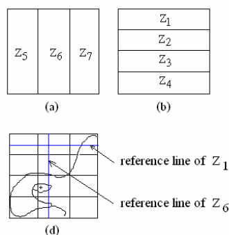
Fig. 4 (a) The zones that use vertical referent lines. (b) The zones that use horizontal referent lines. (d) Two referent lines pass Zones Z_1 and Z_6 that make an attribute to be Feature\_Code\_Z_1 = 1 and Feature\_Code\_Z_6 = 5
