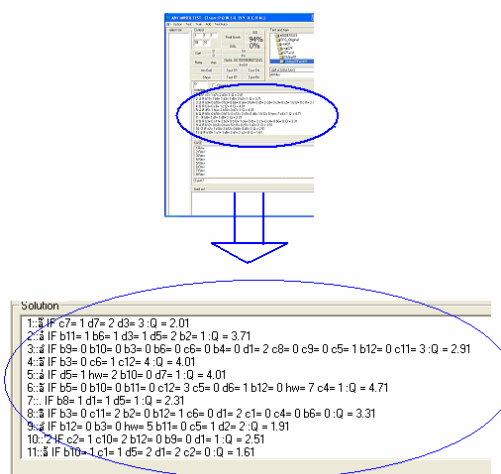
Fig. 13 Example of rule list (a, b and c are three feature end points, Head and feature code. The \bar{a} , \bar{b} , \bar{c} , \bar{d} , \bar{e} , \bar{f} , \bar{g} , and \bar{h} are classes of characters)
