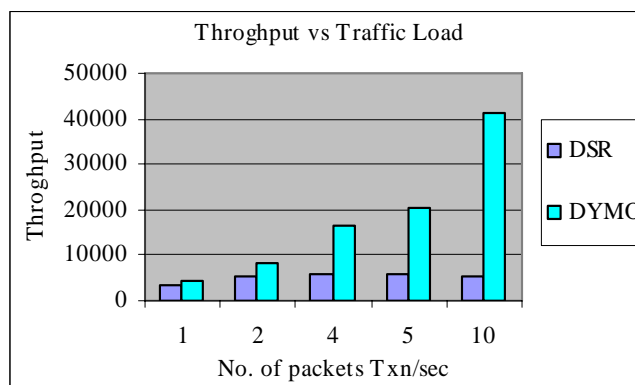
Fig. 2 Throughput Vs Traffic Load
