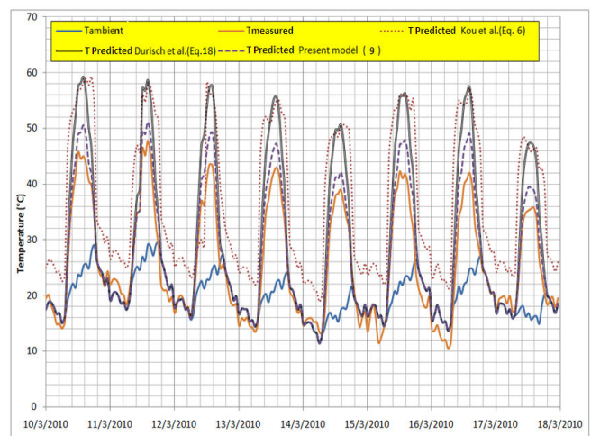
Fig. 7 Measured and modeled PV-cell temperature
