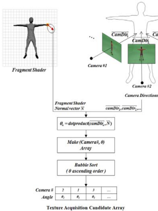
Fig. 3 The process of creation of the texture acquisition candidate array
