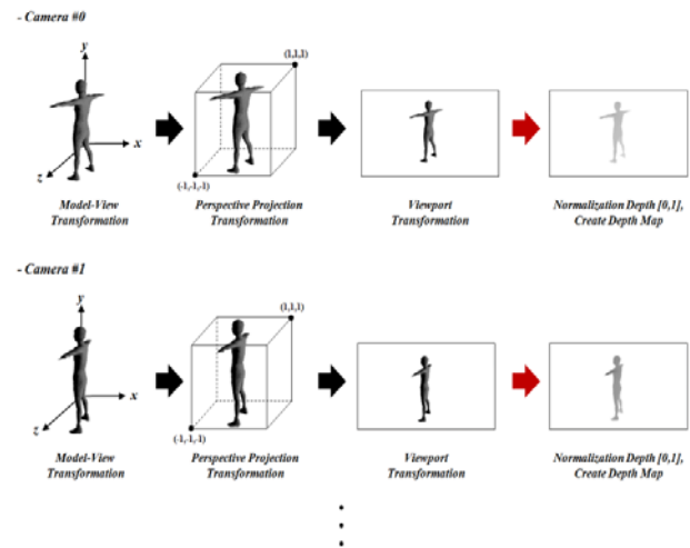
Fig. 2 The depth map generation process for each image
