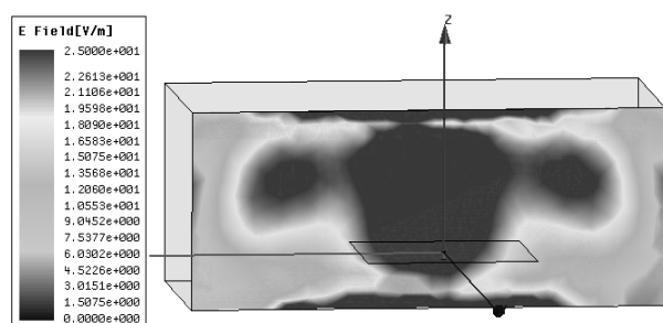
Fig. 1 HFSS analysis output of the electric field distribution inside the cage that was used during the exposure period
