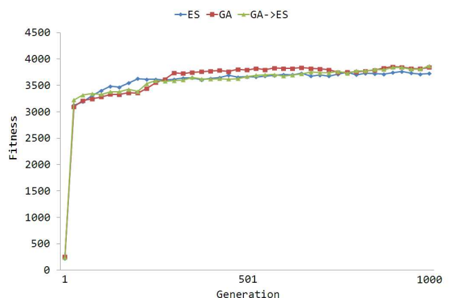
Fig. 7 Result of evolutions by the three algorithms
