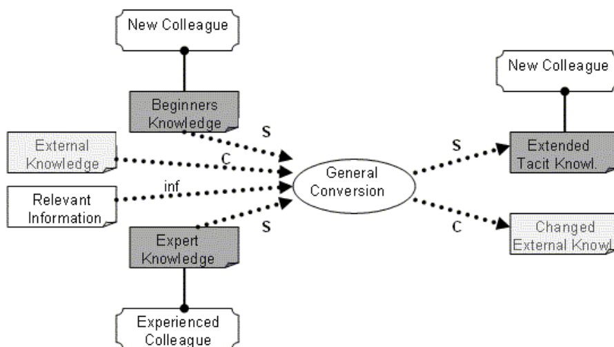
Fig. 4 Supervised learning-by-doing
