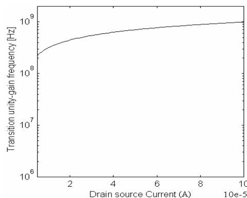
Fig. 9 Unity gain frequency as a function of drain source current in strong inversion region
