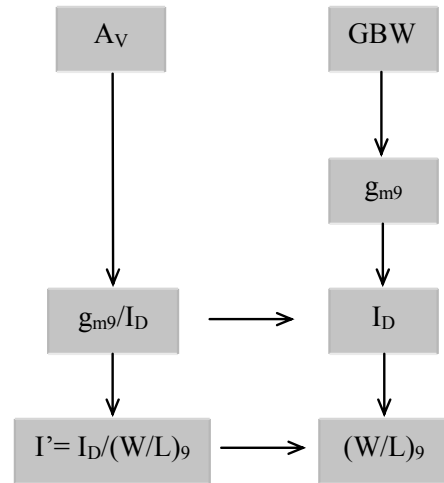
Fig. 2 Design flow
