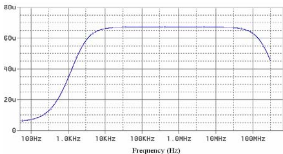
Fig. 7 OTA's transconductance in moderate inversion region
