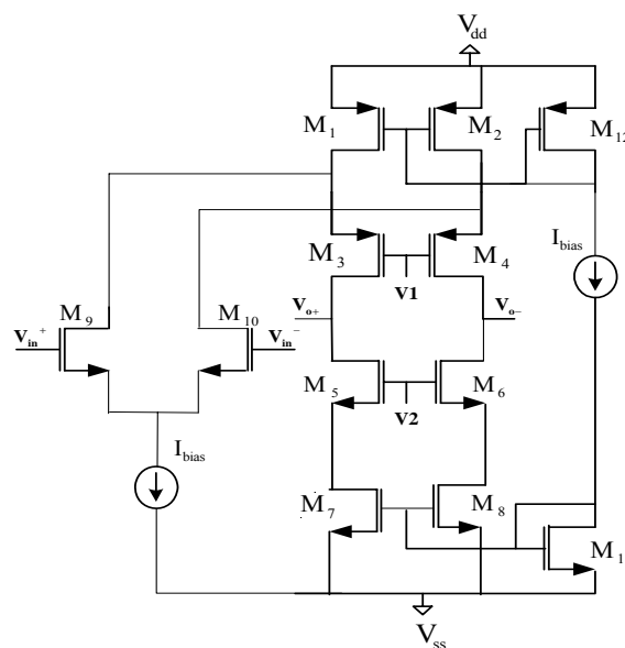
Fig. 1 Folded cascode OTA topology
