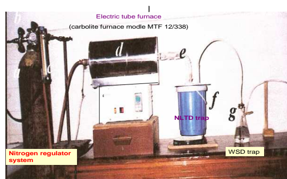
Fig. 1 he apparatus used for pyrolysis of the ten wood species
