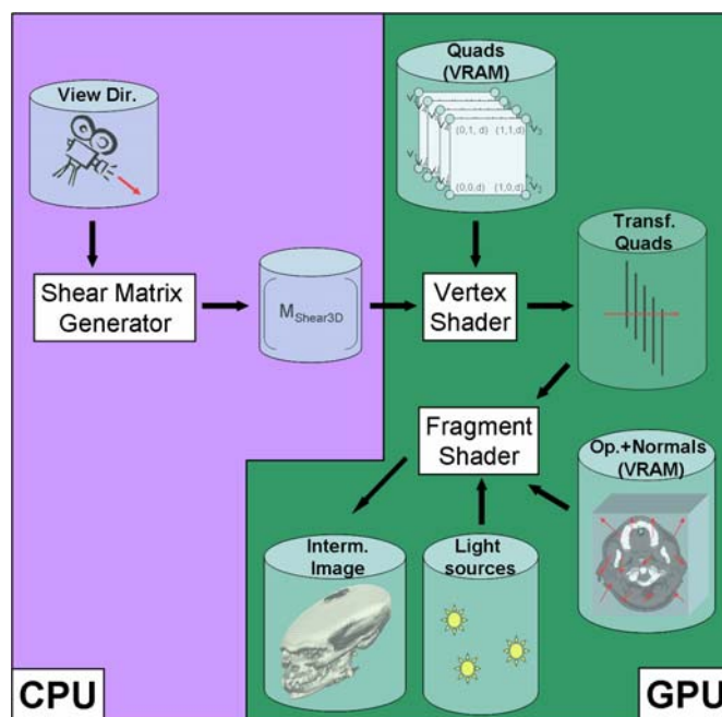
Fig. 5. The first rendering pass consists in applying the shear matrix to the volume slices (represented as a set of quadrilaterals) using the GPU vertex shader. Then, each fragment of those quadrilaterals is shaded on the GPU using the Phong model (Fig. 7), according to the corresponding opacity and normal. The output of the fragment shader is the intermediate, distorted image.
