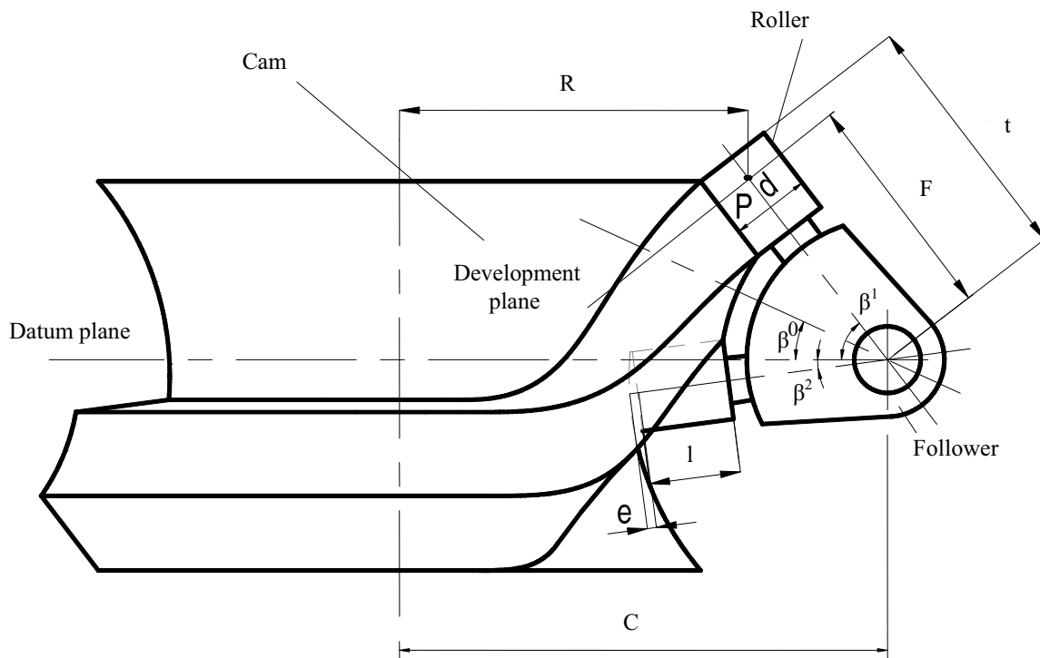
Fig. 2 Globoidal cam- oscillating follower arrangement
