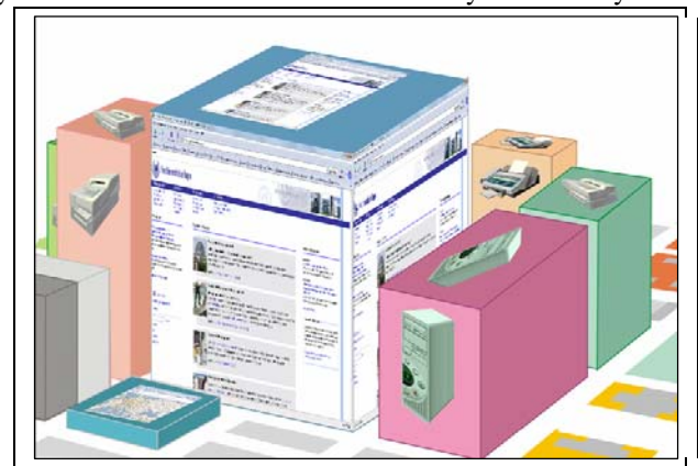
Fig. 4 Network neighborhood
