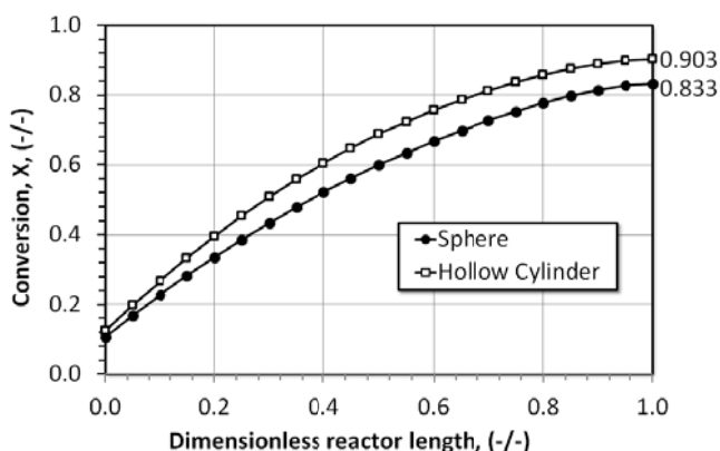
Fig. 3 Conversion profile for the conversion for heterogeneous model using hollow cylindrical catalyst pellet and spherical pellet for (\gamma_o) = 1 for \kappa = 0.5
