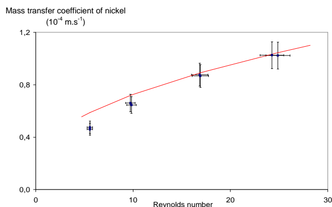
Fig. 5 Mass transfer coefficient of nickel versus Reynolds number for an inlet nickel concentration fixed at 20 \text{ mg.kg}^{-1} ■: experimentally measured and —: calculated from Dwivedi and Upadhyay correlation [12] with D=6.6 \times 10^{-10} \text{ m}^2.\text{s}^{-1}
