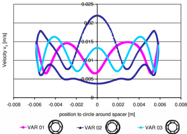
Fig. 9 Velocity v_y progression around spacer
