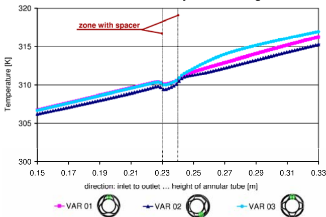
Fig. 6 Temperature progression along the channel – point 1
