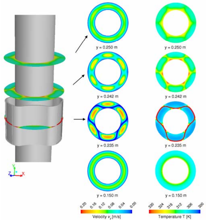
Fig. 3 Flow and temperature fields of spacer VAR 01
