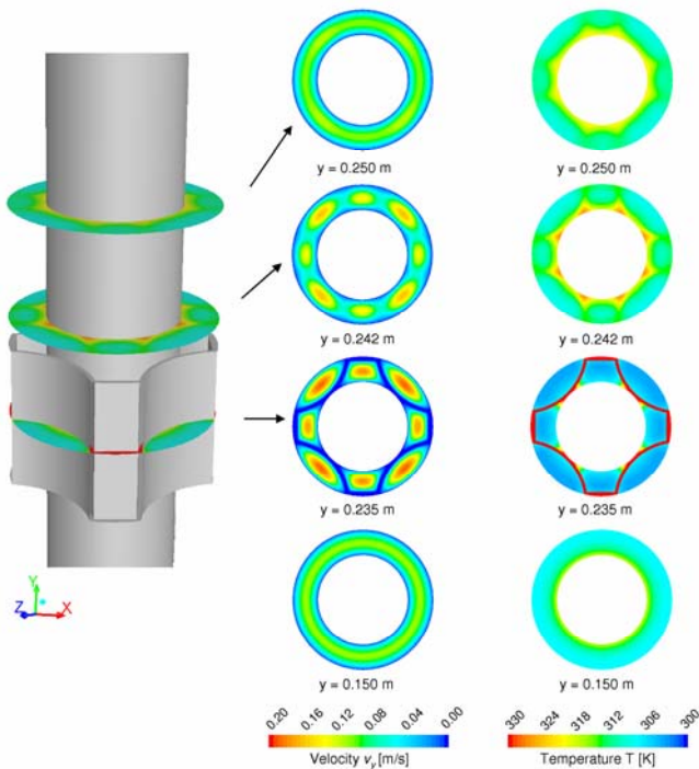
Fig. 5 Flow and temperature fields of spacer VAR 03
