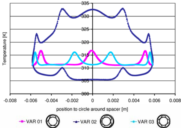
Fig. 8 Temperature progression around spacer
