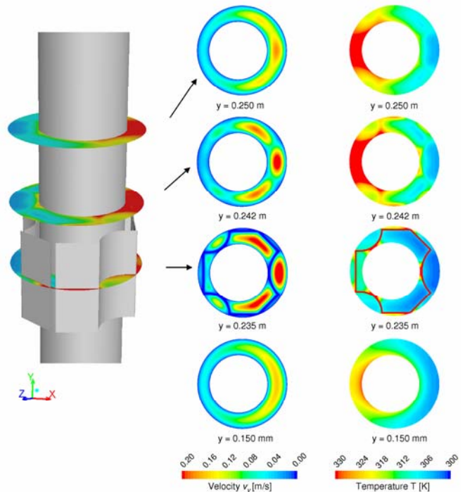
Fig. 4 Flow and temperature fields of spacer VAR 02
