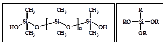
Fig. 1 Polydimethylsiloxane and alkyltrialkoxysilane
