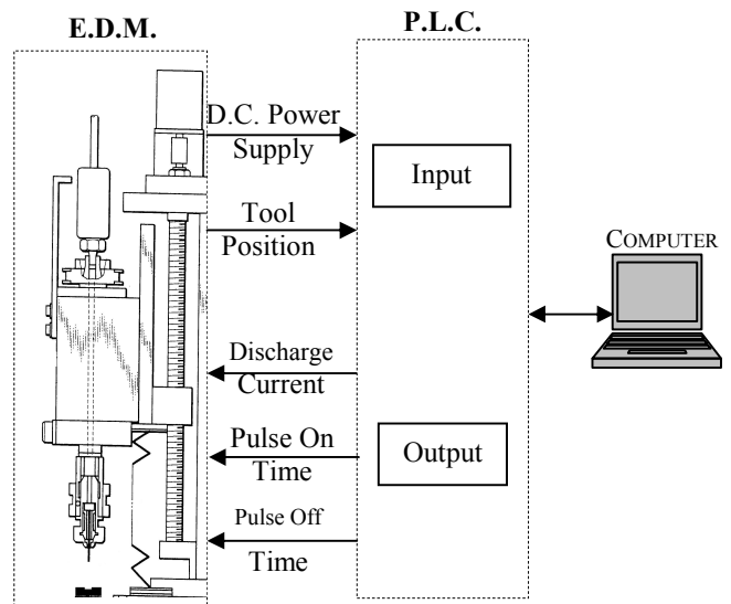
Fig. 1 Schematic diagram of EDM-PLC interface
