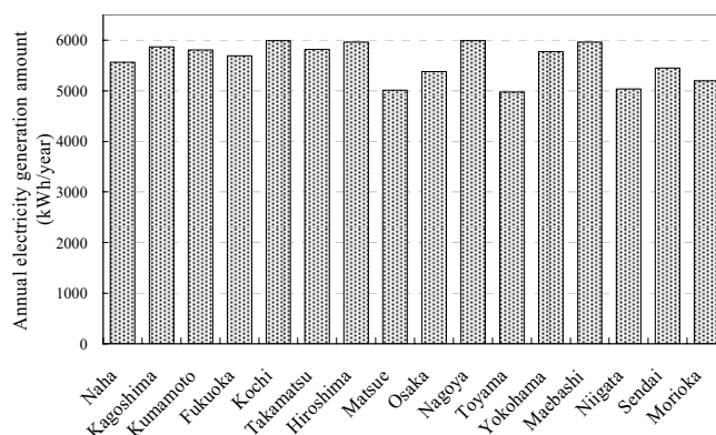
Fig.7 Annual electricity generation amount
