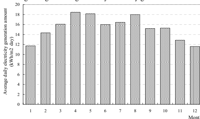
Fig. 6 Whole country average daily electricity generation amount
