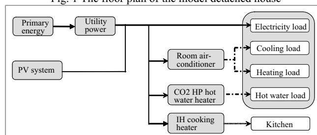
Fig. 2 the energy system with the photovoltaic system
