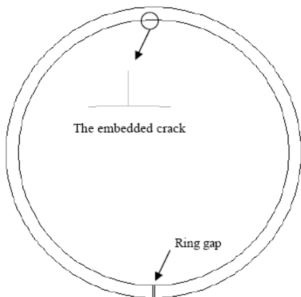
Fig. 4 2D model of the first compression ring
