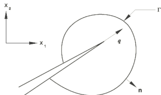
Fig. 1 Contour for evaluation of the J-integral
