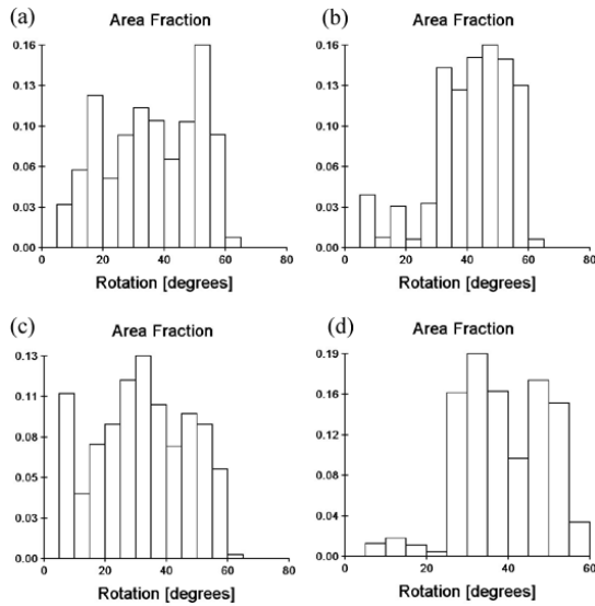
Fig. 4 Frequency histograms of grain or subgrain misorientation taken from the specimens deformed at 850°C under the strain rate of 1 \times 10^{-3}/s . (a) gauge and (b) grip parts, and that of 3 \times 10^{-5}/s , (c) gauge and (d) grip parts, respectively
