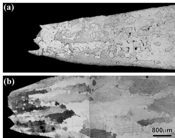
Fig. 8 Optical micrographs taken from surfaces of specimens of (a) binary and (b) ternary alloys fractured at 850°C under the strain rate of 5×10 -4 /s
