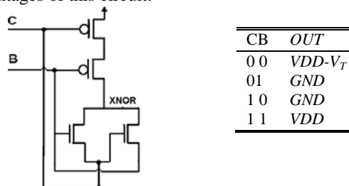
Fig. 7 The XNOR with four transistors.
