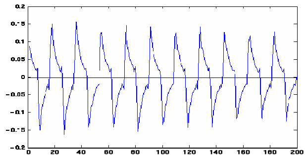
Fig. 5 Output signal of Vmike smart sensor through an AC coupling circuit
