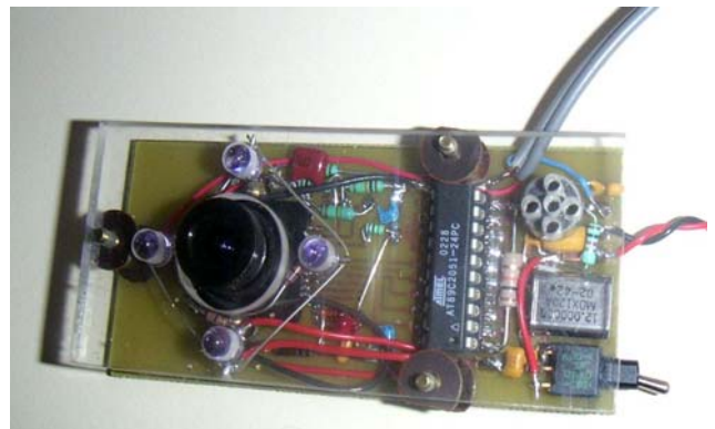
Fig. 9 Vmike Prototype
