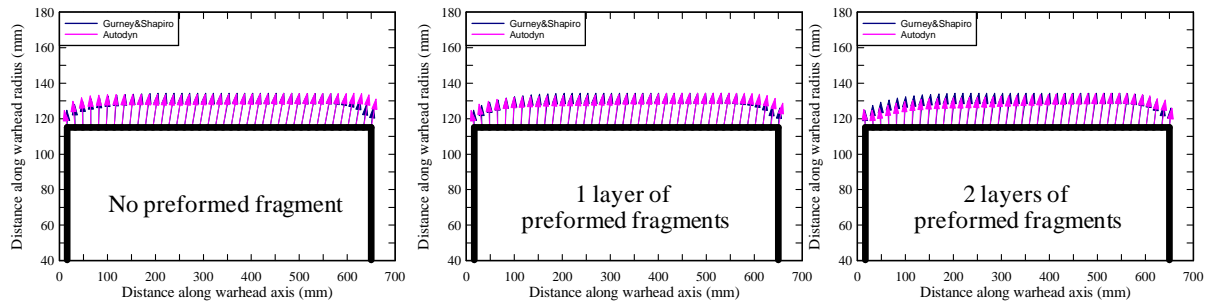
Fig. 6 Comparison of velocity vectors of casing obtained from analytical calculation and FE simulation
