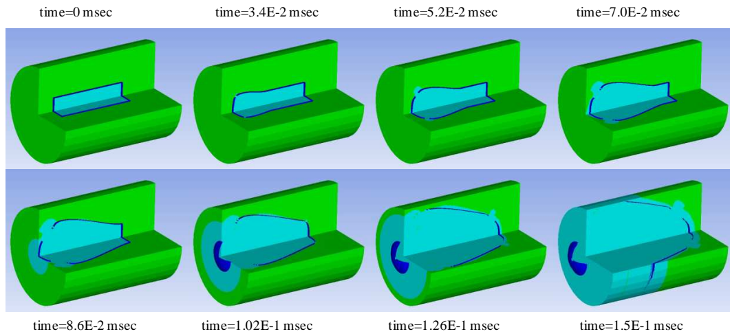
Fig. 4 Warhead explosion processes
