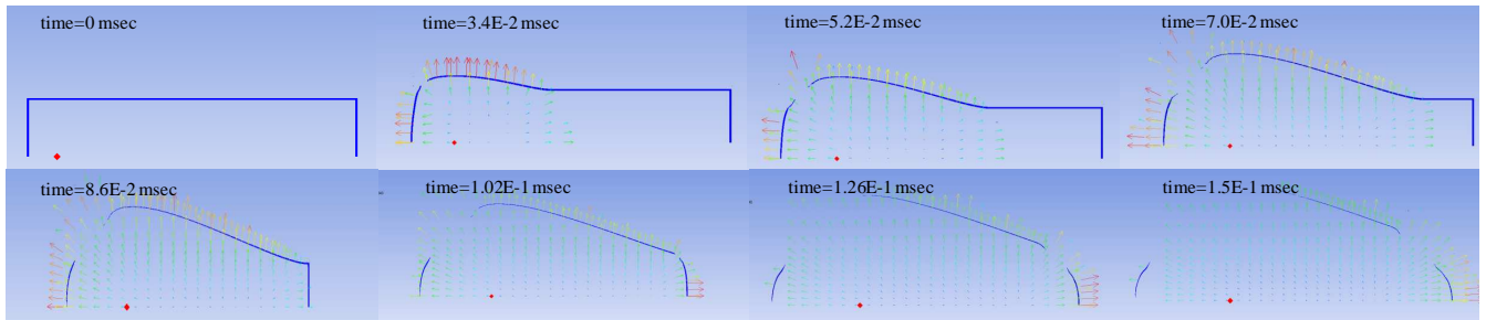
Fig. 5 Velocity vectors of warhead casing and TNT
