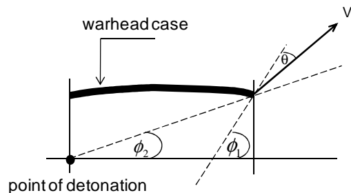
Fig. 1 Spray angle of fragment
