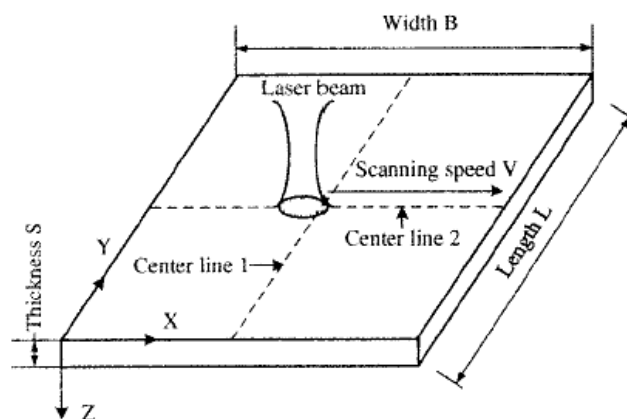
Fig. 1 Schematic diagram of the LBF Process [5]
