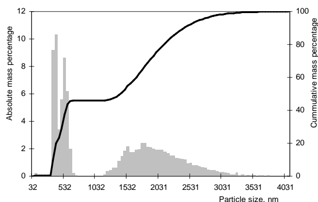
Fig. 1 Particle size distribution of zeolite particles
