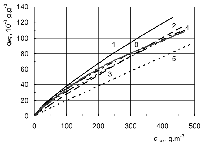
Fig. 5 Adsorption isotherms of nickel on zeolite for the set of NaCl dosages NaCl dosage: 0 – 0 \text{ kg.m}^{-3} , 1 – 1 \text{ kg.m}^{-3} , 2 – 2 \text{ kg.m}^{-3} , 3 – 5 \text{ kg.m}^{-3} , 4 – 10 \text{ kg.m}^{-3} and 5 – 100 \text{ kg.m}^{-3}
