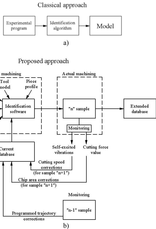
Fig. 2 Identification scheme a) Classical approach b) Proposed approach
