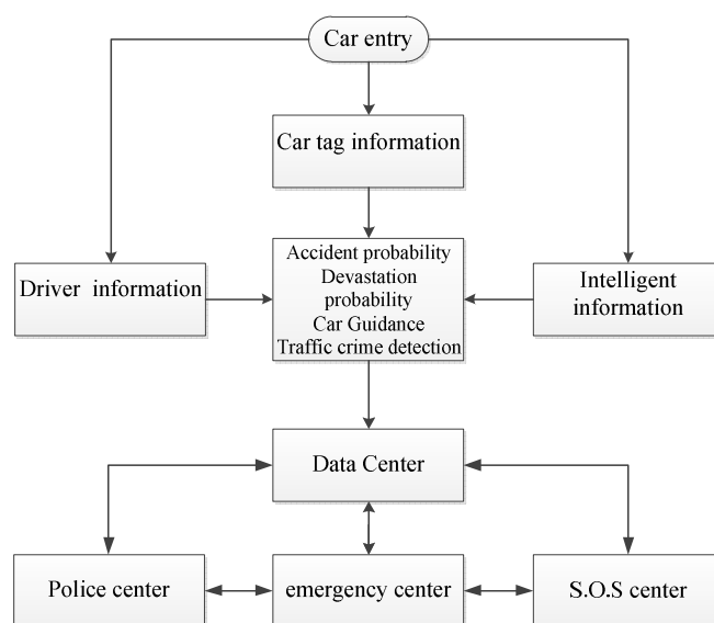
Fig. 4 Flowchart of system
