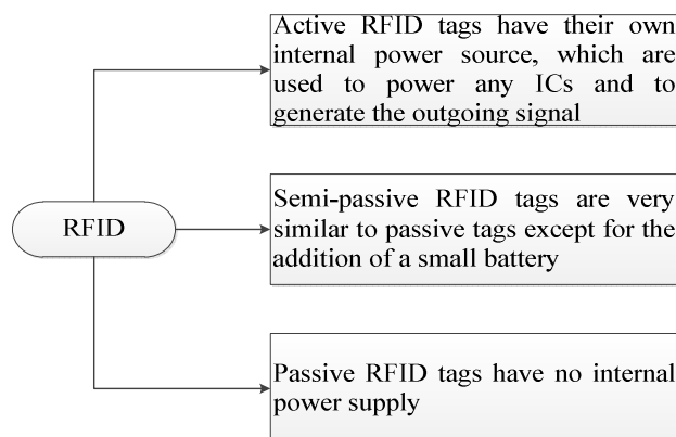
Fig. 2 RFID types
