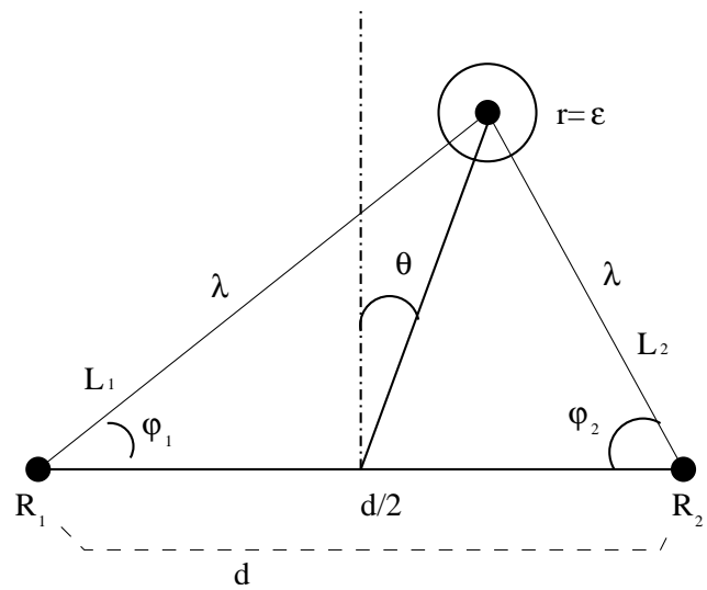
Fig. 1. Two Receivers and one Sender
