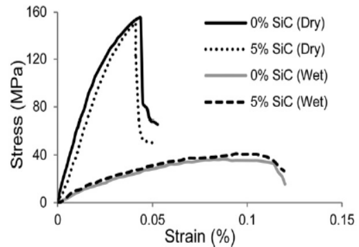
Fig. 13 Stress-strain curves of RCF/epoxy filled with 0 and 5 wt% n-SiC in dry and wet conditions
