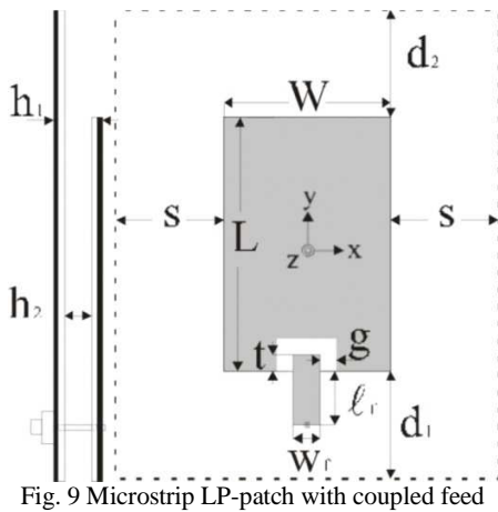
Fig. 9 Microstrip LP-patch with coupled feed
