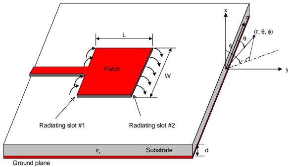
Fig. 1 Rectangular microstrip antenna
