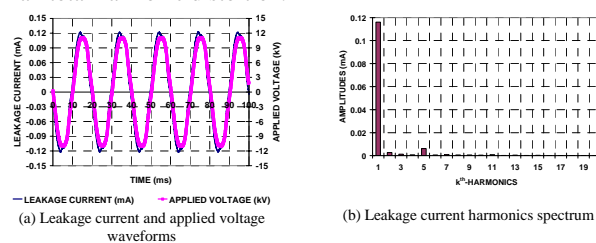
Fig. 3. The waveforms of wet polluted insulator
