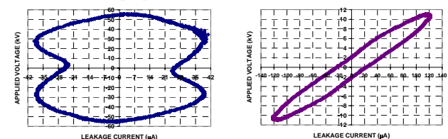
(a) Dry condition (71% RH), phase angle 74.9° (b) Wet condition (99% RH), phase angle 12.2°
