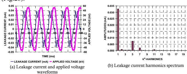
Fig. 2. The waveforms of dry polluted insulator
