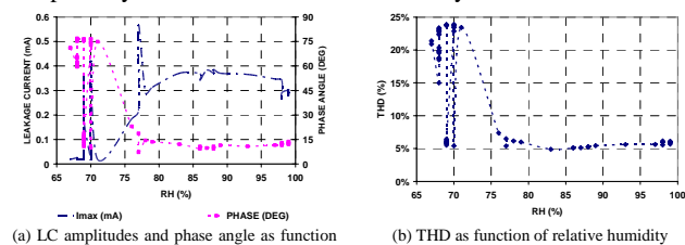
Fig. 4. LC, phase angle (a) and THD (b) as function of relative humidity
