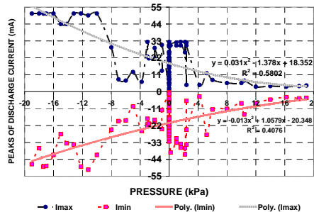
Fig. 10. Experimental results of (+) and (-) peaks of discharge current as function of pressure
