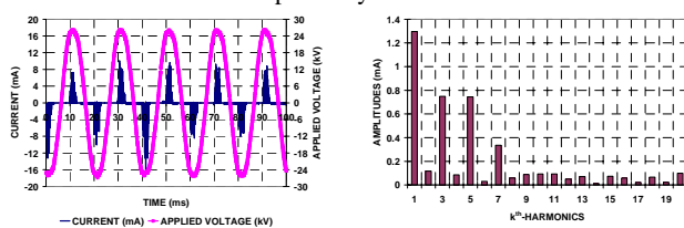
(a) Discharge current and applied voltage waveforms (b) Discharge current harmonics spectrum
