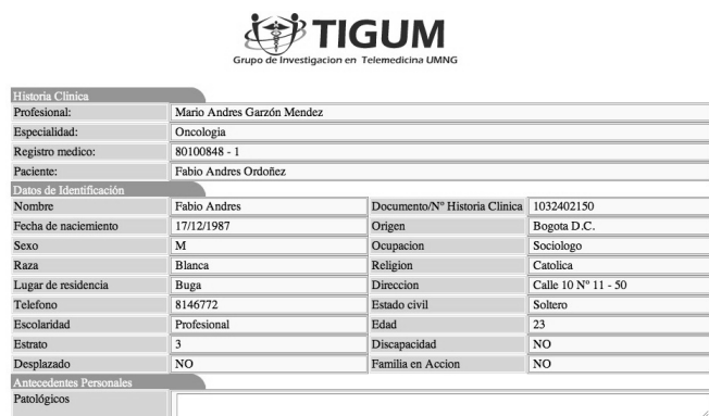
Fig. 13 System GUI
