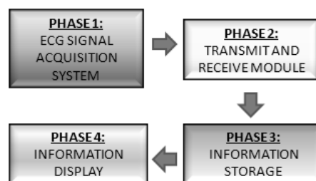
Fig. 4 Methodology
