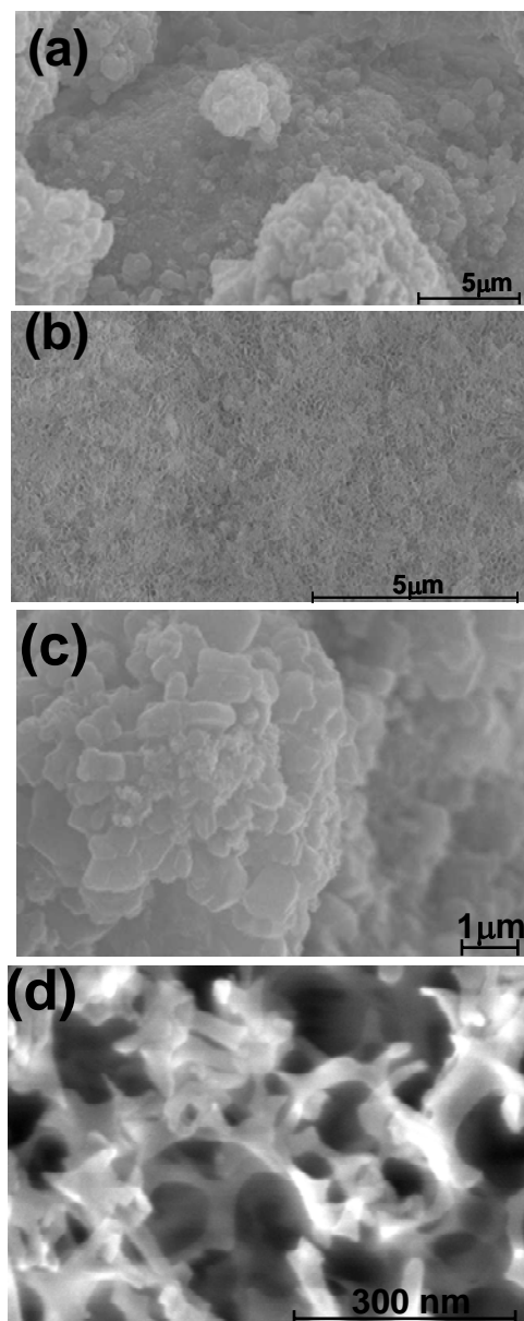
Fig. 3 SEM image of (a) Silicone rubber/SiO 2 coating on aluminum surface (b) RF-sputtered PTFE coating deposited on an anodized aluminum surface
