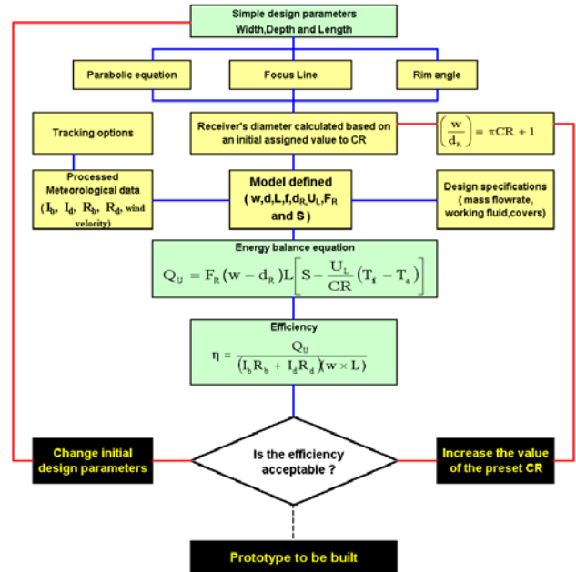
Fig. 2 A flowchart outlining the design process
