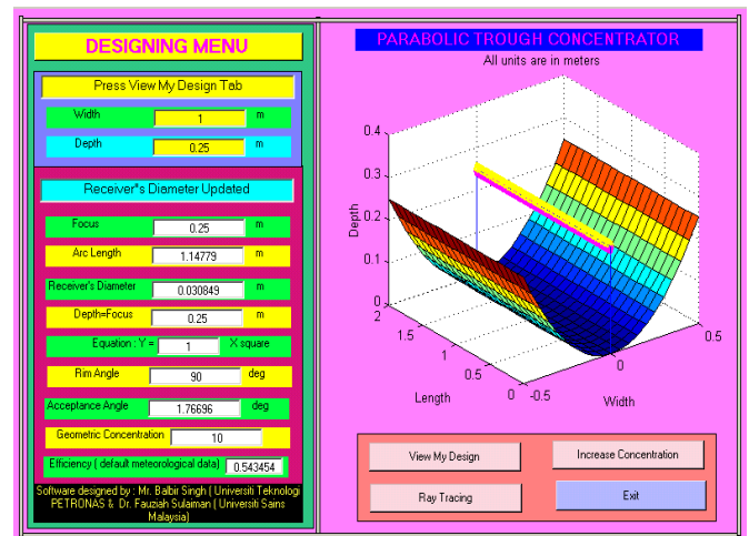
Fig. 3 A snapshot of the design menu and a 3-D model generated by the simulation program in the MATLAB environment
