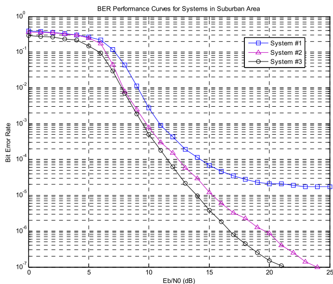
Fig. 4. Bit error probability versus energy per bit/noise power spectral density ( E_b/N_0 ) for system #1, system #2, and system #3 with DBPSK, over Rician-multipath fading channel ( K factor= 1 ) with Bi-Gaussian Doppler PSD.
