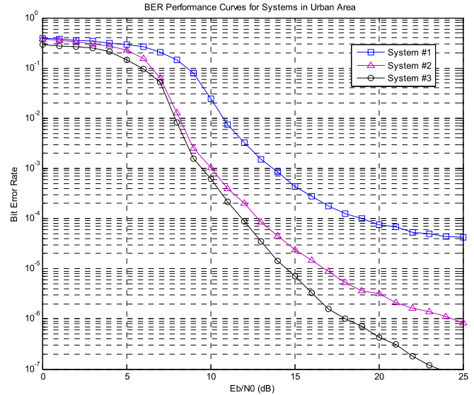
Fig. 2. Bit error probability versus energy per bit/noise power spectral density ( E_b/N_0 ) for system #1, system #2, and system #3 with DBPSK, over Rayleigh-multipath fading channel with Bi-Gaussian Doppler PSD.
