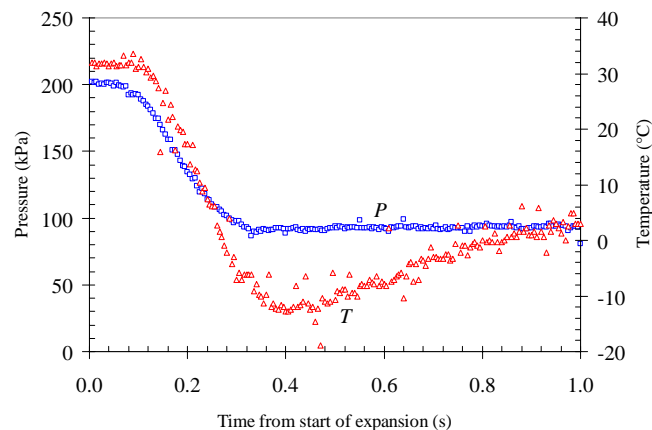
Fig. 2 Typical variation of temperature and pressure during the expansion of a turbulent mixture of iso-octane-air
