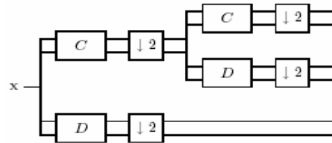
Fig. 1 Multi-rate Filter bank
