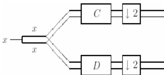
Fig. 2 Multiwavelet Filter banks with “repeated input”
