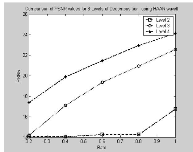
Fig. 8 Comparison of PSNR values for 3 levels of decomposition using "HAAR" wavelet for Fingerprint-A
