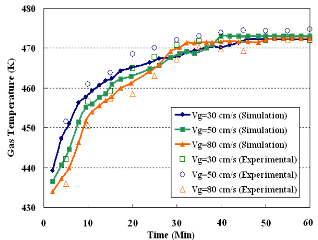
Fig. 8 Comparison of experimental and computational results for gas temperatures at different gas velocities ( z=50 cm)
