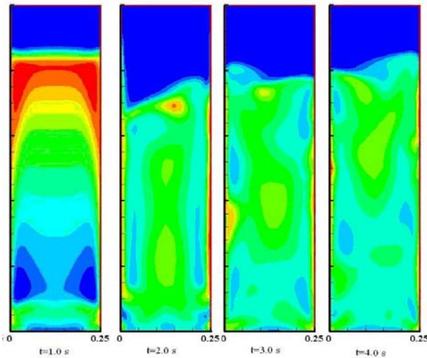
Fig. 3 Simulated solid volume fraction contours in the 2D bed ( V_g = 50 \text{ cm/s} , drag function: Syamlal-O'Brien)
