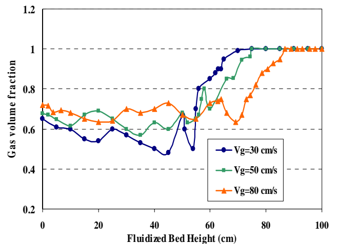
Fig. 5 Simulation results for gas volume fraction at t=5\text{s} (Syamlal-O'Brien drag model)
